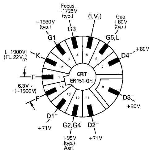
Voltages at the CRT socket
